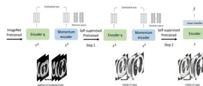
Figure 1 structure of Self-trans + DenseNet-169 [31] .
